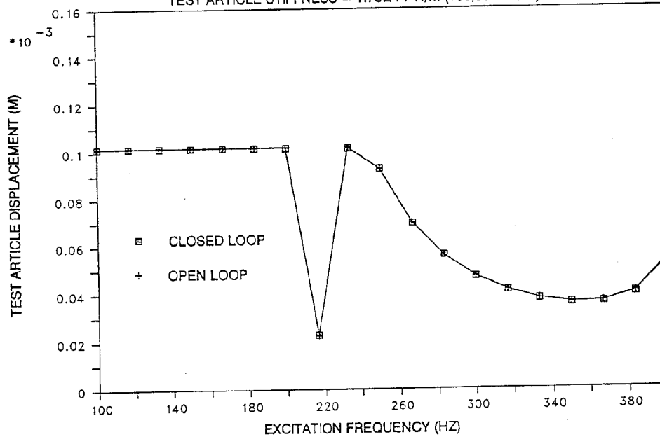
Figure 10. Maximum Response at Test Article, Test Article Stiffness = 100,000 lb/in.
