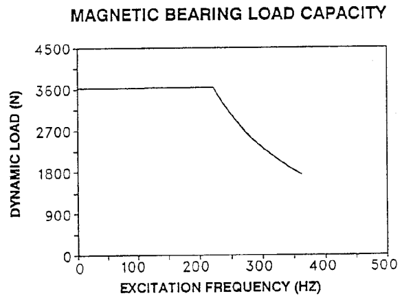
Figure 4. Magnetic Bearing Load Capacity vs. Excitation Frequency
