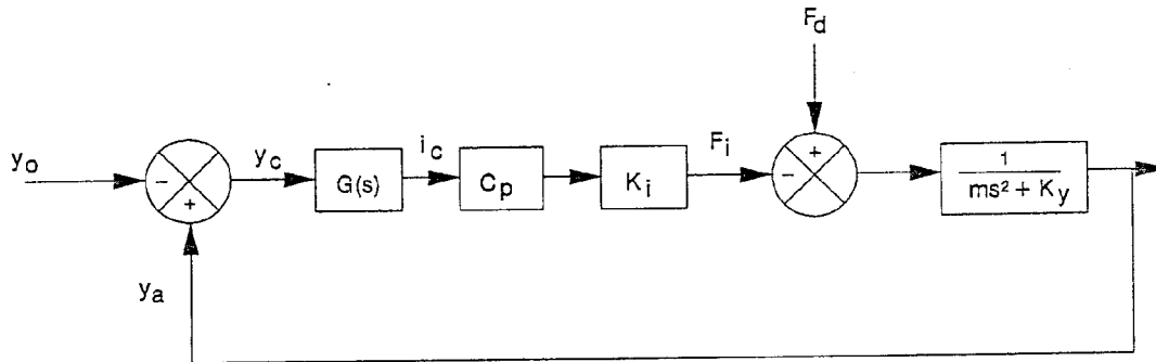
Figure 5. Magnetic Bearing Control Diagram
