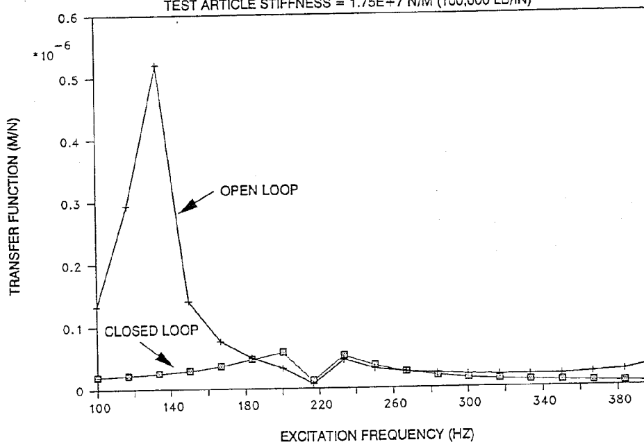
Figure 9. Transfer Function Amplitude, Response at Test Article due to Force at Magnetic Bearing, Test Article Stiffness = 100,000 lb/in.
