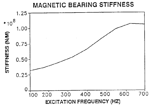
Figure 2. Magnetic Bearing Stiffness Coefficient vs. Excitation Frequency
