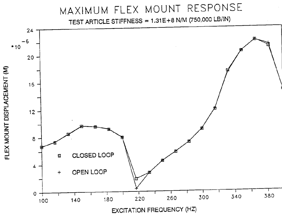
Figure 14. Maximum Response at Flex Mount Load Sensing Element, Test Article Stiffness = 750,000 lb/in.
