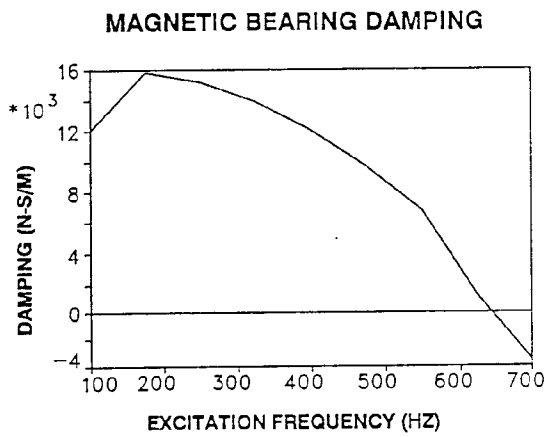
Figure 3. Magnetic Bearing Damping Coefficient vs. Excitation Frequency
