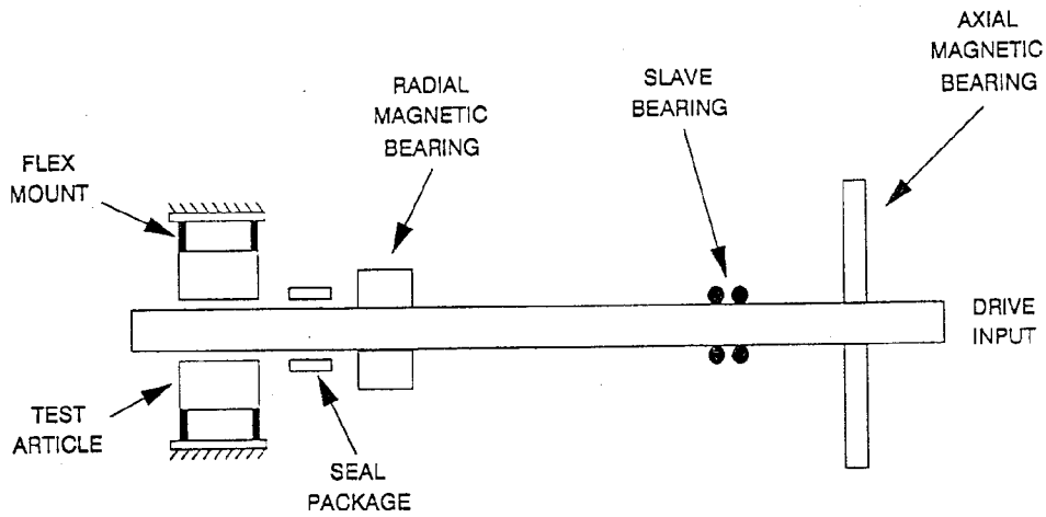
Figure 6. Schematic of Rocketdyne Multifunction Tester
