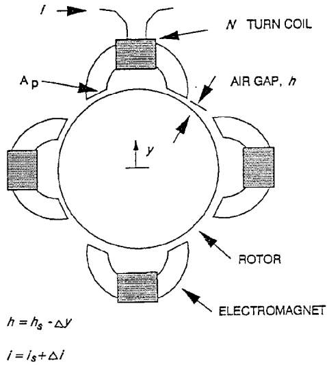
Figure 1. Magnetic Bearing Schematic
